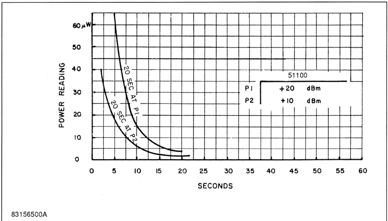
Figure 4-2 Diode Sensor Decay
