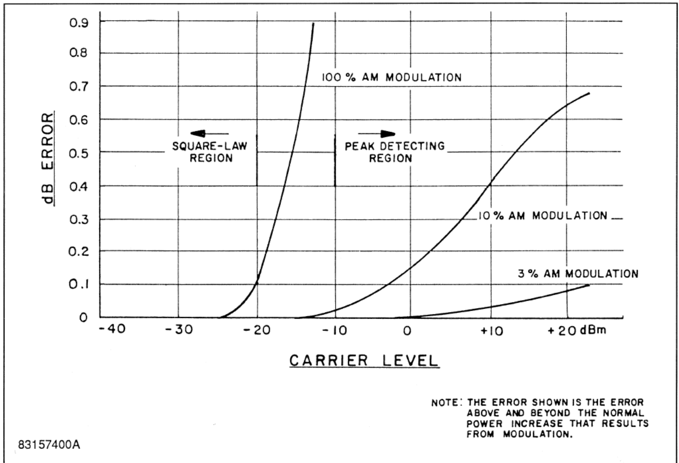
Figure 4-12. Error Due to AM Modulation (51013 Diode Sensor)
